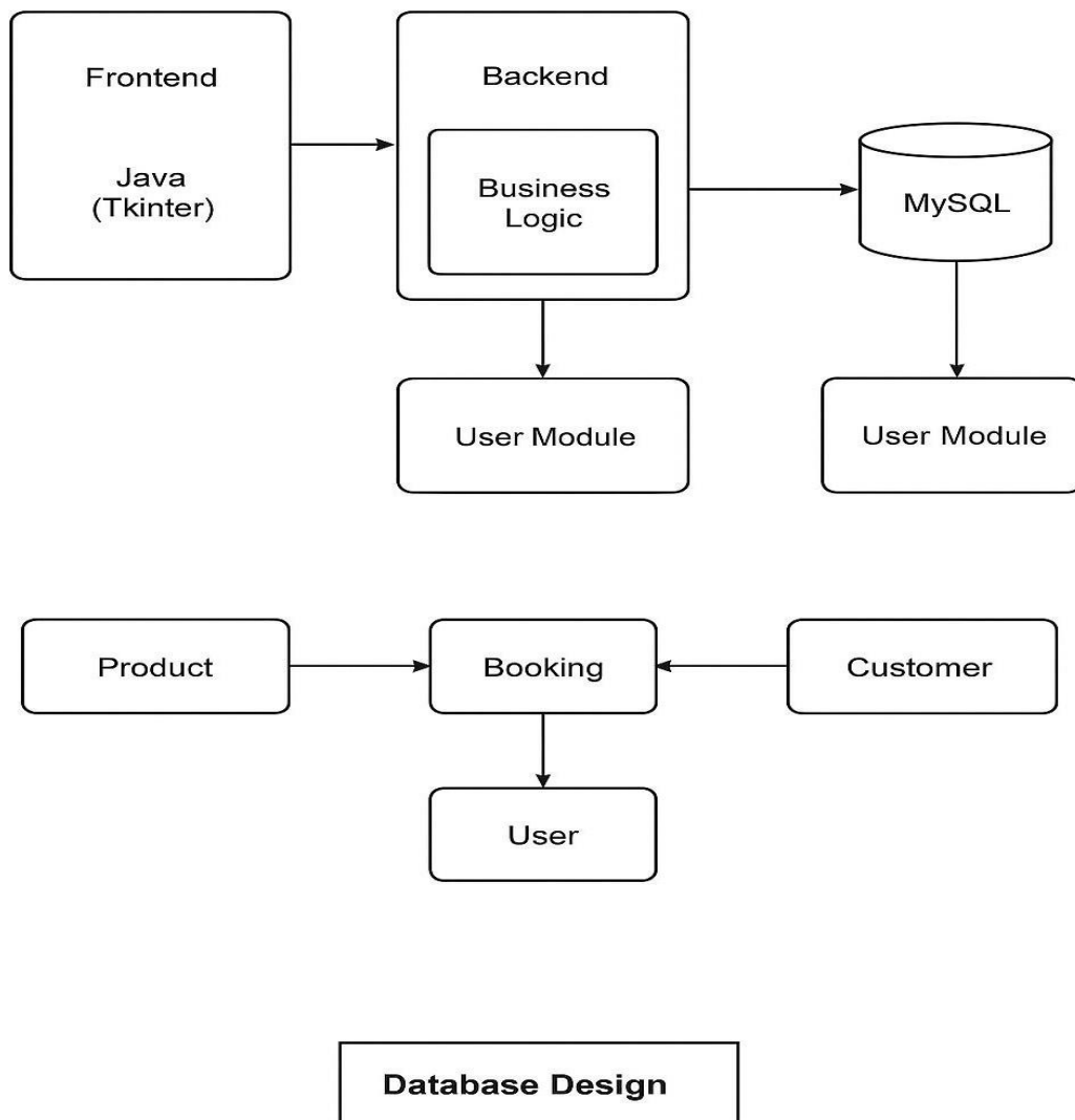
FIG.1.1.DATABASE ARCHITECTURE
